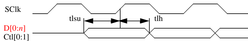
Figure 5-11 — PHY to link transfer waveform at the link
