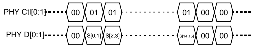
Figure 5-5 — Status timing
