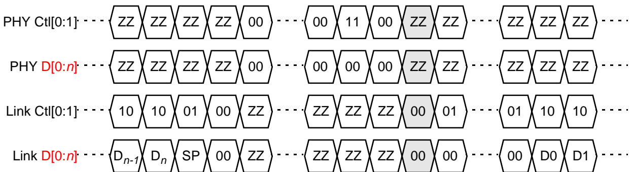
Figure 5-6 — Transmit timing
