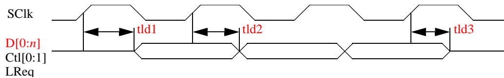
Figure 5-12 — Link to PHY transfer waveform at the link
