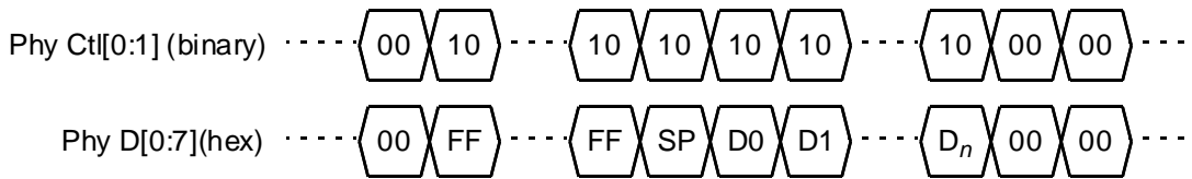
Figure 5-7 — Receive timing
