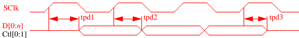
Figure 5-9 — PHY to link transfer waveform at the PHY
