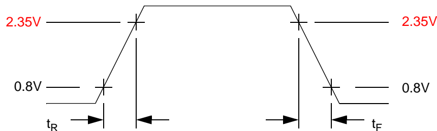
Figure 5-8 — Signal levels for rise and fall times
