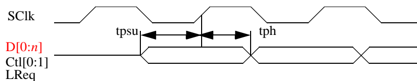
Figure 5-10 — Link to PHY transfer waveform at the PHY
