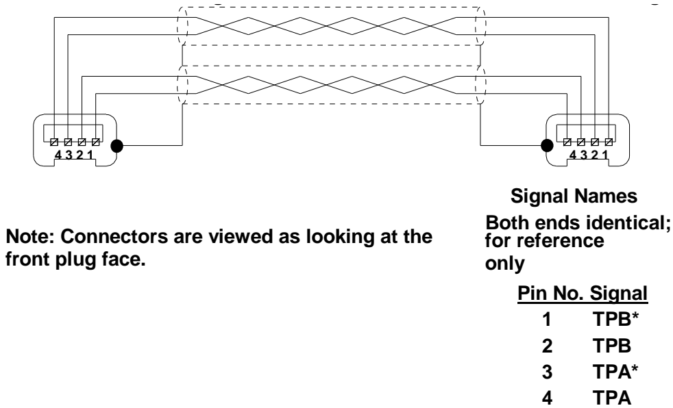
Figure 4-11—Cable assembly and schematic (alternate connectors)
